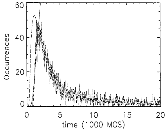
Fig. 3. Distribution of the times at which the sudden rise in \Psi^2 occurs; an illustration of this rise for a sample run was given in Fig. 2. Solid curve: fit of early-time data to Eq. (2); dashed curve: fit of late-time data to the phenomenologically altered Eq. (2). The curves cross at t_2 .
