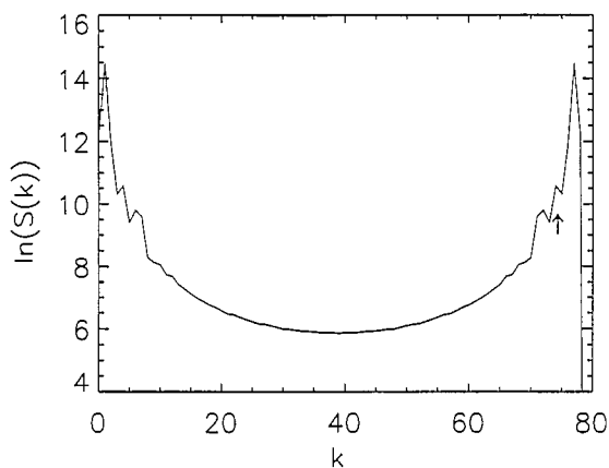
Fig. 8. The logarithm of the structure factor S(k) given by Eq. (7) vs. k_y , where \hat{y} is along the mean direction of the steps for simulated data such as depicted in Fig. 7, at T = 0.624\epsilon/k_B . The distinct periodicity along the step edges is evident from the satellite peak, indicated by an arrow.
