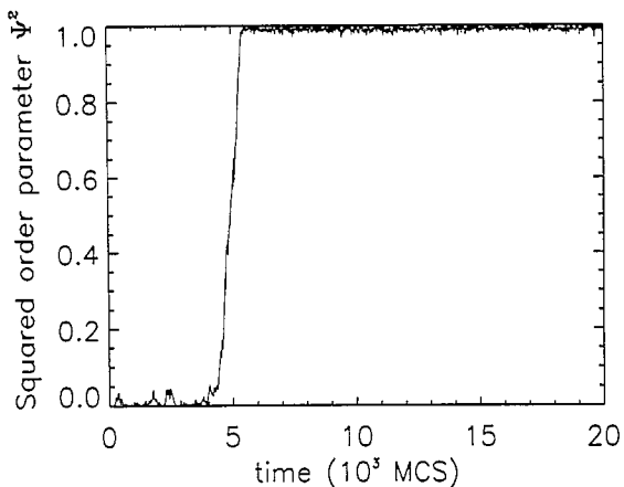
Fig. 2. \Psi^2 vs. t from a single Monte Carlo run at T = 0.624\epsilon/k_B , showing the rapid "zipping together" of neighboring steps once they make contact.
