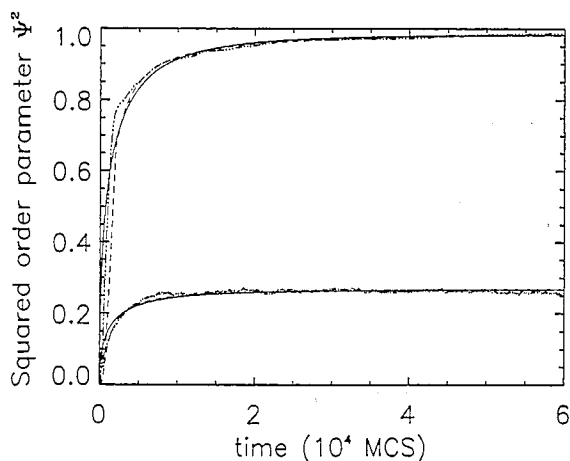
Fig. 1. \Psi^2 vs. t at temperatures 1.404\epsilon/k_B and 0.624\epsilon/k_B , where \epsilon is the energy of a kink or, equivalently, a unit length of step. The dashed-dot line gives the results of Monte Carlo simulations, while the solid line is the best fit to the two-parameter functional form \Psi^2 = A[1 - \exp(-\sqrt{t/t_0})] . The dashed line is the best fit to the functional form of Eq. (4).
