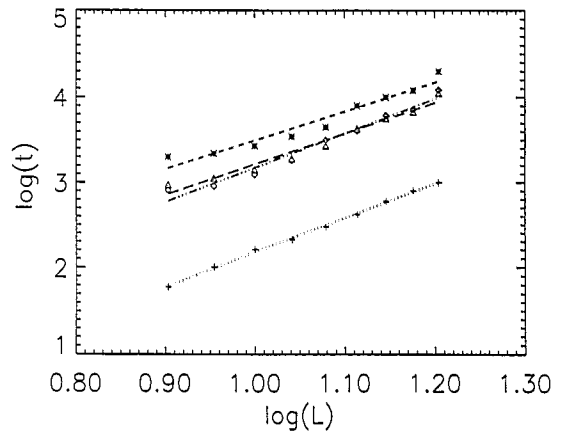
Fig. 4. Logarithm of the various time constants t vs. logarithm of the average distance L between single height steps (i.e., 1/\tan(\phi) , where \phi is the misorientation angle), at T = 0.624\epsilon/k_B . The plus signs indicate the values of t_0 obtained by fitting Eq. (1) to our simulation results. The corresponding linear fit has a slope s = 4.36 \pm 0.06 . The asterisks, triangles, and diamonds indicate the values of t_1 , t_2 , t_3 , respectively, obtained by fitting Eq. (4) to our simulation data. The corresponding best linear fits are shown. Their respective slopes are 3.37 \pm 0.30 , 3.62 \pm 0.25 and 4.03 \pm 0.25 . This result and those of Bartelt et al. [17] suggest a relation of the form of Eq. (6).
