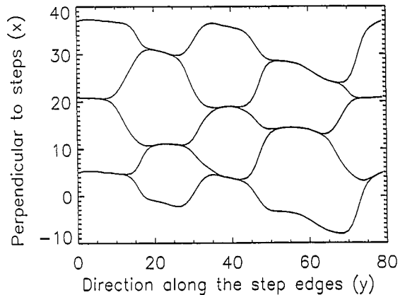
Fig. 7. Sample of a long time average of the step structure as viewed from a direction normal to the terraces. This simulation was done at T = 0.624\epsilon/k_B , and atoms were only allowed to move along the step edge, implying thereby constant \Psi (0 in this case). The four steps were initially straight and uniformly spaced at a distance \ell = 8 apart. To help visualize the configuration, a fifth step is depicted here; it is just the first step, shifted by L_x , as dictated by the screw-periodic boundary conditions.
