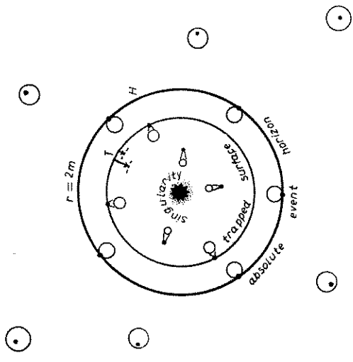
Fig. 4. - Spatial view of spherical «black hole» (Schwarzschild solution).
