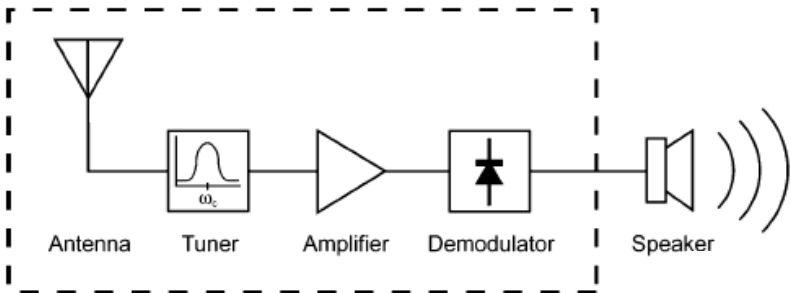
All-in-one nanotube radio
